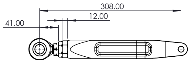
MIN ADJUSTMENT
