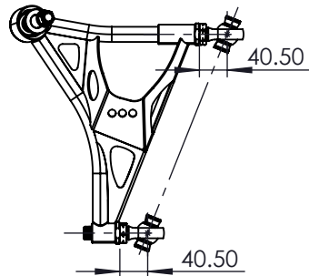
MIN LENGTH
